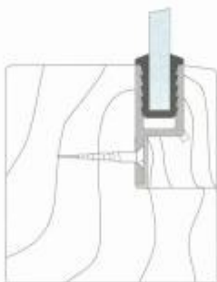
The Glaze-Guard 'h' Profile should be securely fitted to the existing frame.
