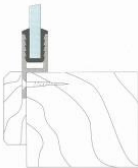
The Glaze-Guard 'h' Profile should be securely fitted to the existing frame.
