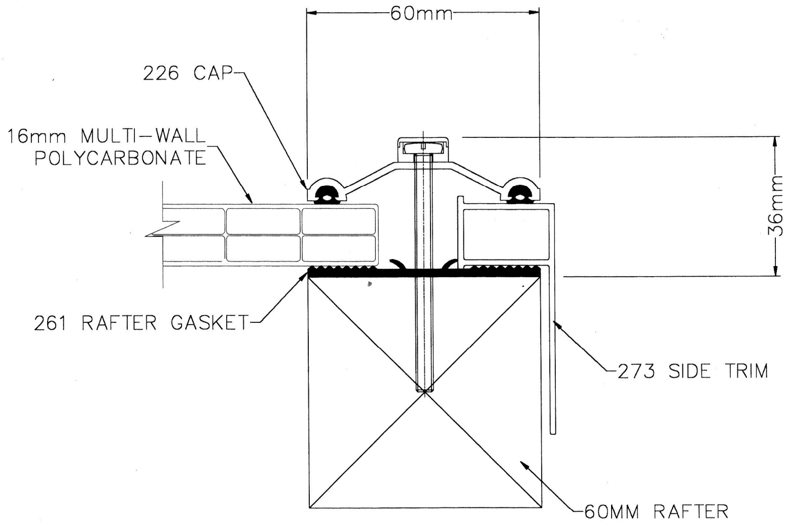
226/261 RAFTER GASKET WITH 273 SIDE TRIM
