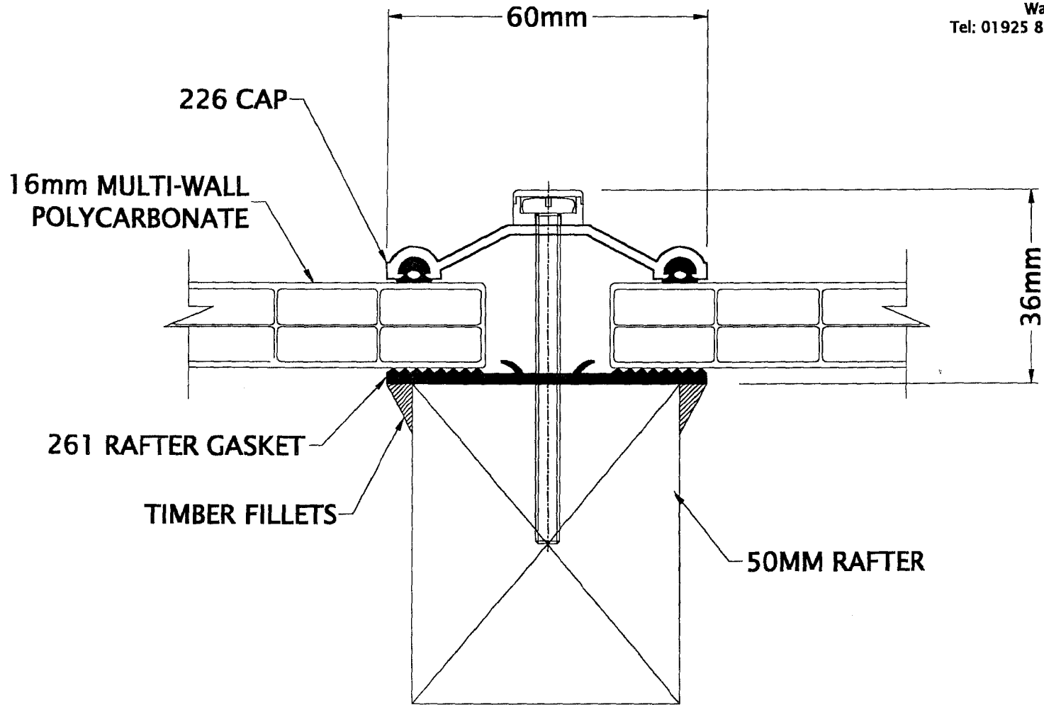
226/261 RAFTER GASKET WITH TIMBER FILLETS
