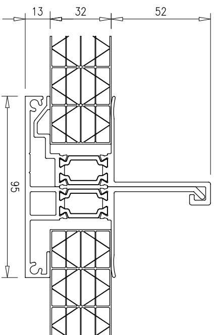
SECTION THROUGH 32mm THERMAL MULTI-LINK BAR
