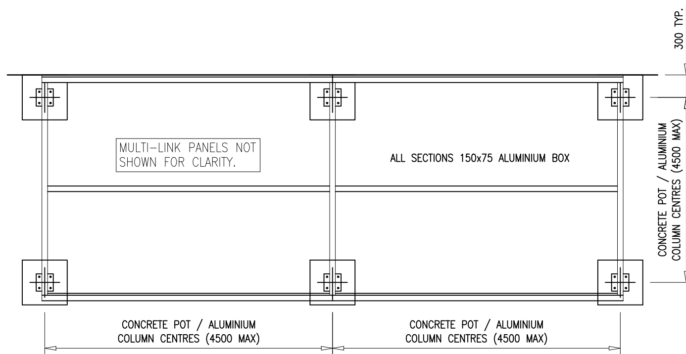
PLAN VIEW ON STRUCTURE SCALE 1:50
