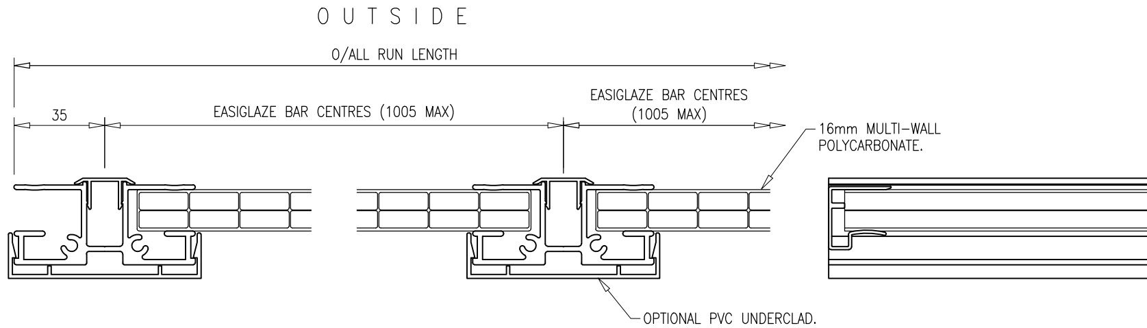
SECTION THROUGH 16mm EASIGLAZE PANELS
