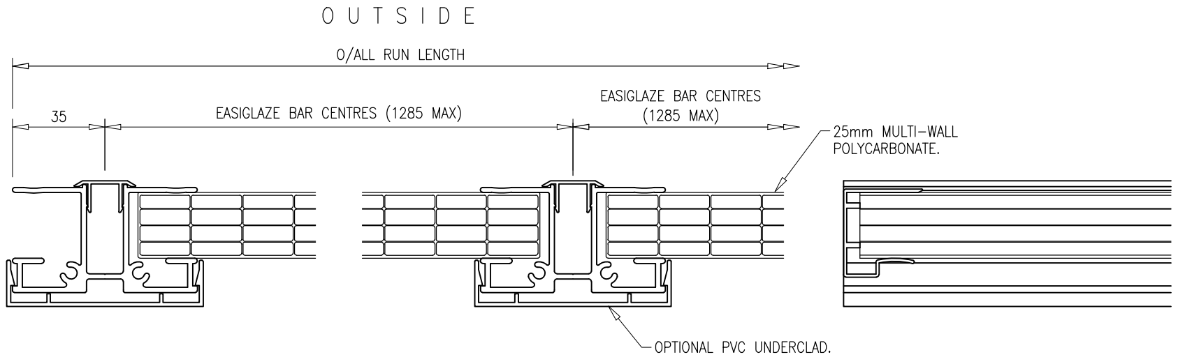
SECTION THROUGH 25mm EASIGLAZE PANELS
